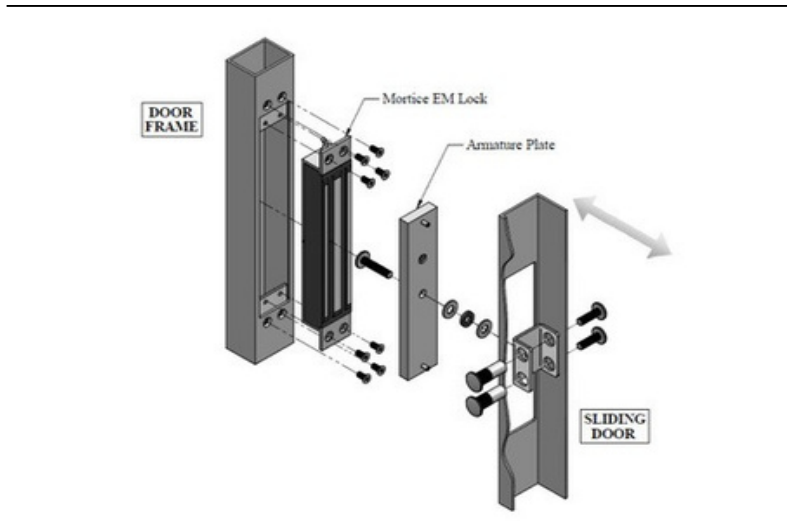
Explode View
