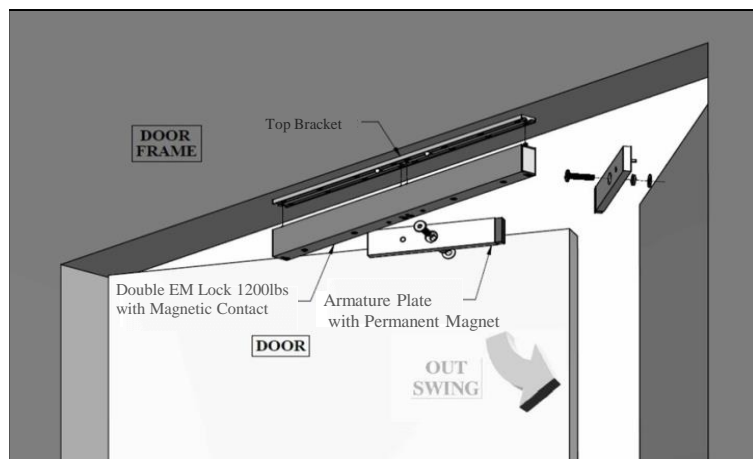
Explode View
