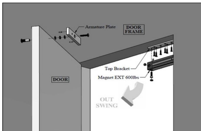
Explode View
